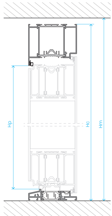
Vertical cross-section
