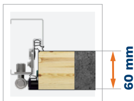
PERFOTHERM 60 Türrahmen
