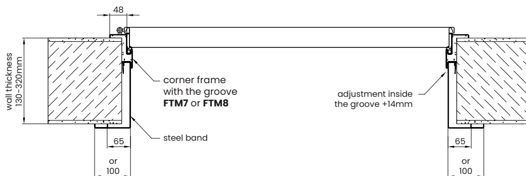
HORIZONTAL CROSS-SECTION
