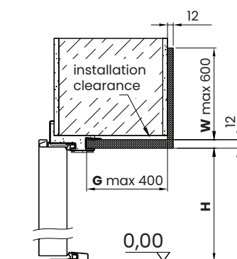
VERTICAL CROSS-SECTION
