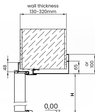
VERTICAL CROSS-SECTION
