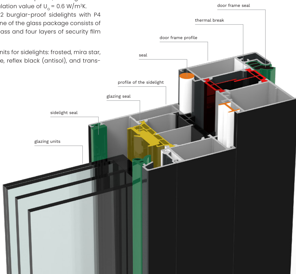
GLAZING UNIT FOR SIDE PANEL (example of the color of the components)
