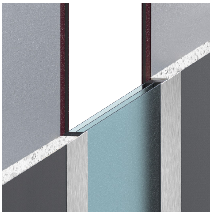
GLAZING UNIT OF THE DOOR LEAF
