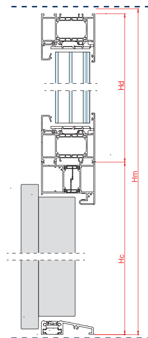
TOP GLAZED PANEL WITH DOOR VERTICAL CROSSECTION
