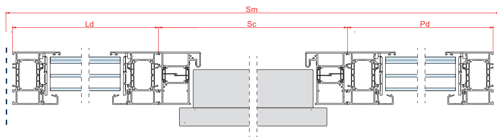
SIDE GLAZED PANEL WITH DOOR HORIZONTAL CROSSECTION
